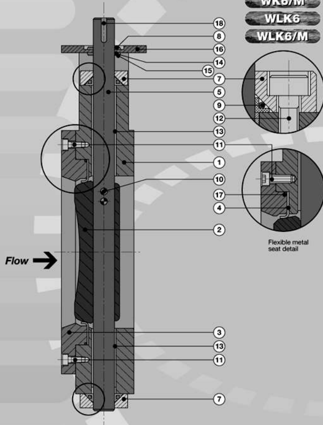
WK/M Section view
