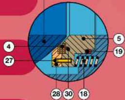
Lamellar seal seat details
